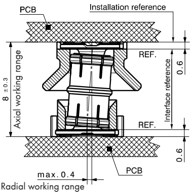
Working range
