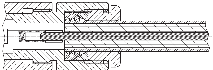
Cable entry for corrugated copper tube cables
