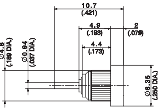
Fig. 2 (press-in)
