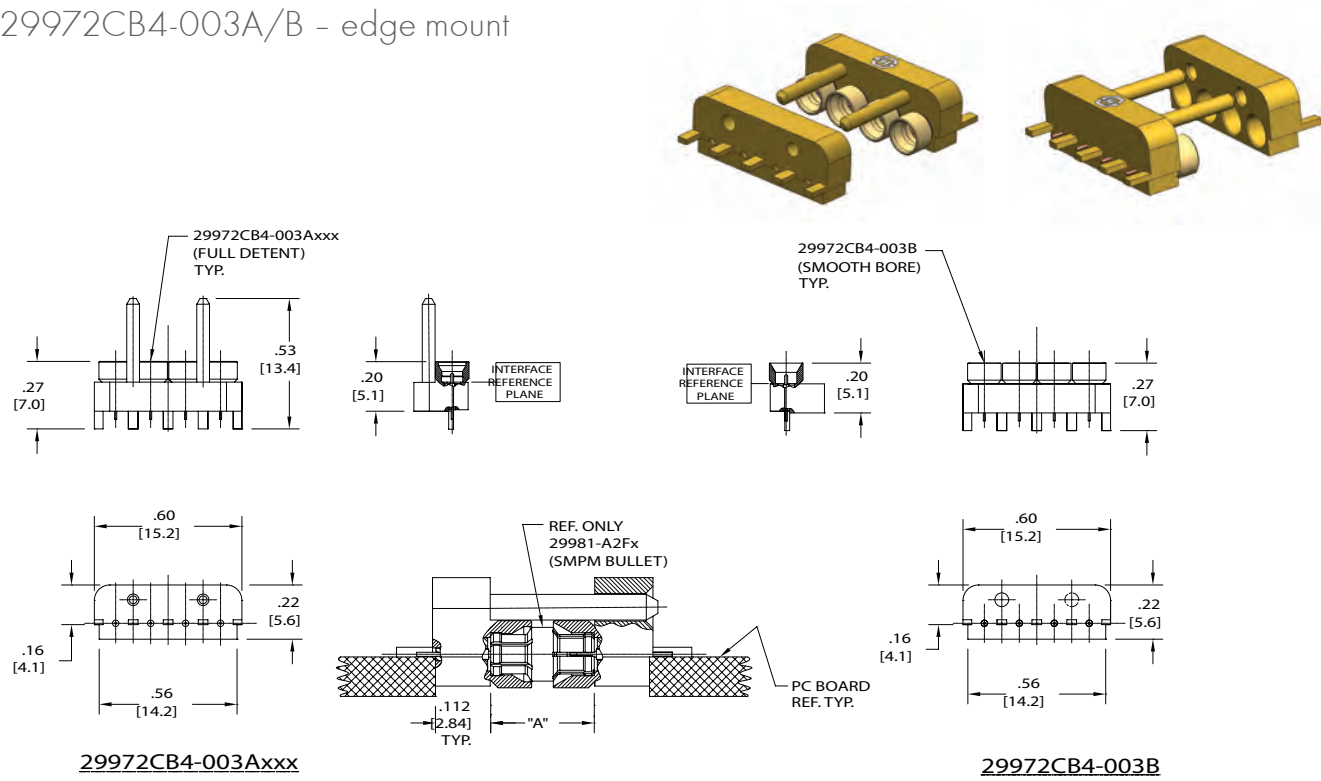
4 CHANNEL PC BOARD TO PC BOARD CONNECTOR BLOCKS WITH BULLET
