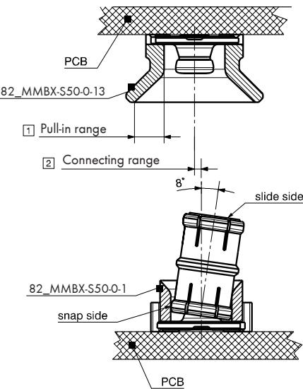
Connecting range
