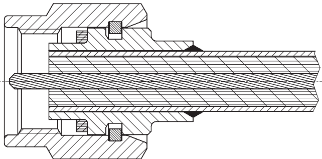
Solderless cable entry, clamp cone
